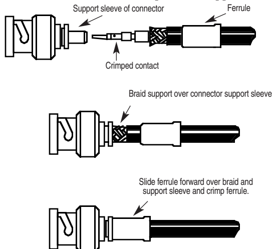
Figure 2. Typical assembly procedure.
