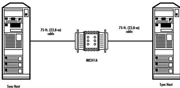
Figure 4-1. Installing the SME-NPR.
