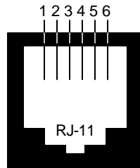
RJ-11 (Two-Wire)
