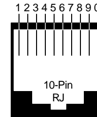
RS-232 Serial 10-Pin RJ Connector
