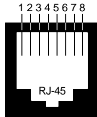
RJ-45 (Two-Wire)
