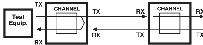
Figure 2-4. Local Aggregate Loopback.
