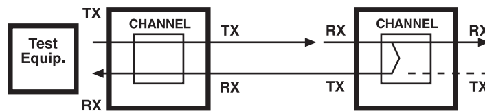
Figure 2-2. Remote Channel Loopback.
