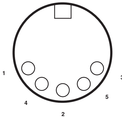
Figure 2-6. Power Connector Pinout.
