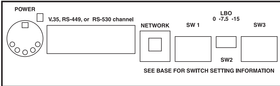
Figure 2-5. Rear-Panel Connections.
