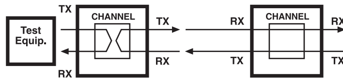
Figure 2-3. Local Channel Loopback.
